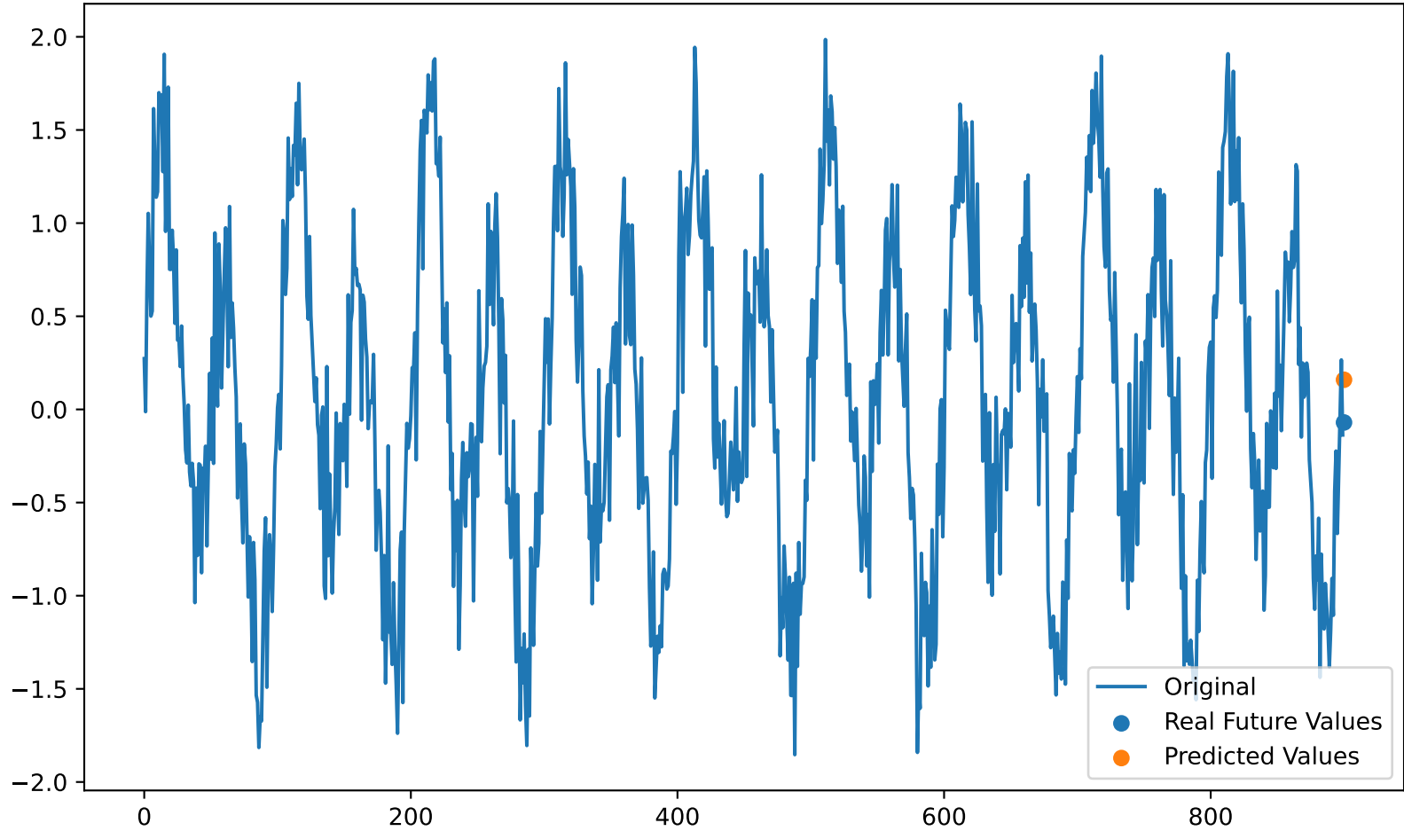
ARIMA( p = 7, q = 7 )
